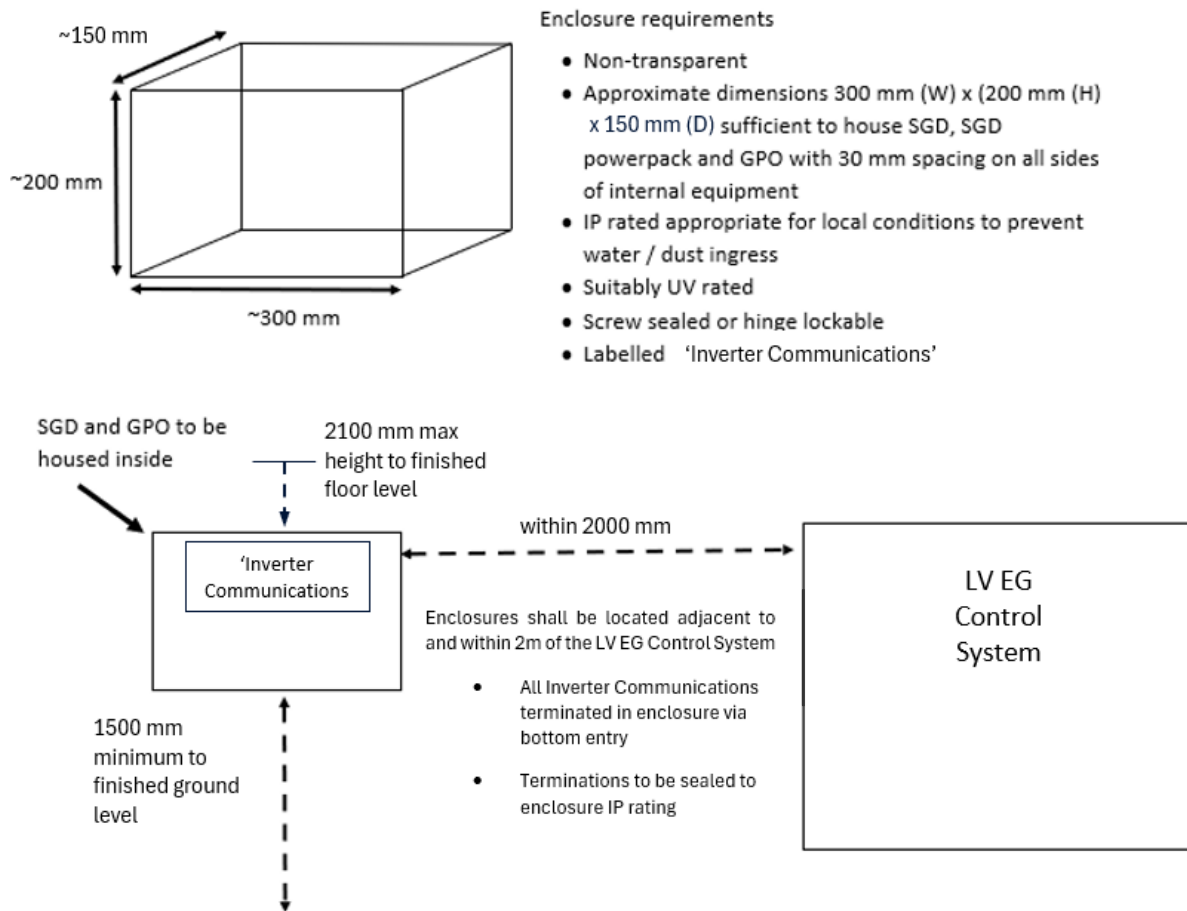
Figure 12: SGD Enclosure Installation Diagram (Indicative)
